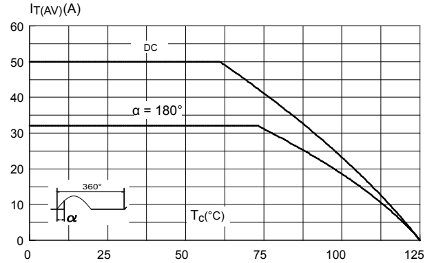
Figure 2. Average on-state current versus case temperature
