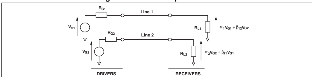
Figure 17. Crosstalk phenomena
