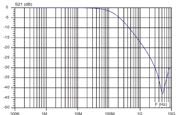
Figure 7. S21 attenuation
