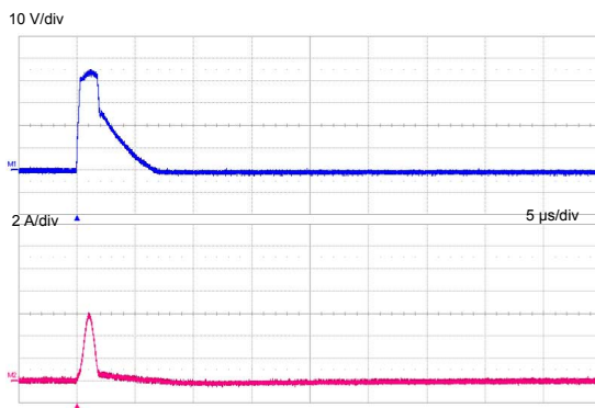
Figure 8. ISO 7637-3 slow transient positive pulse (VS = +85 V)
