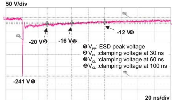
Figure 6. JESD response to IEC 61000-4-2 (-8 kV contact discharge)
