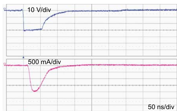
Figure 10. Response to ISO 7637-3 Pulse 3a (U_s = -150 V)
