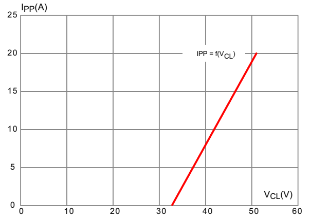
Figure 12. TLP measurements
