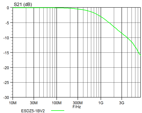
Figure 7. S21 attenuation measurement result
