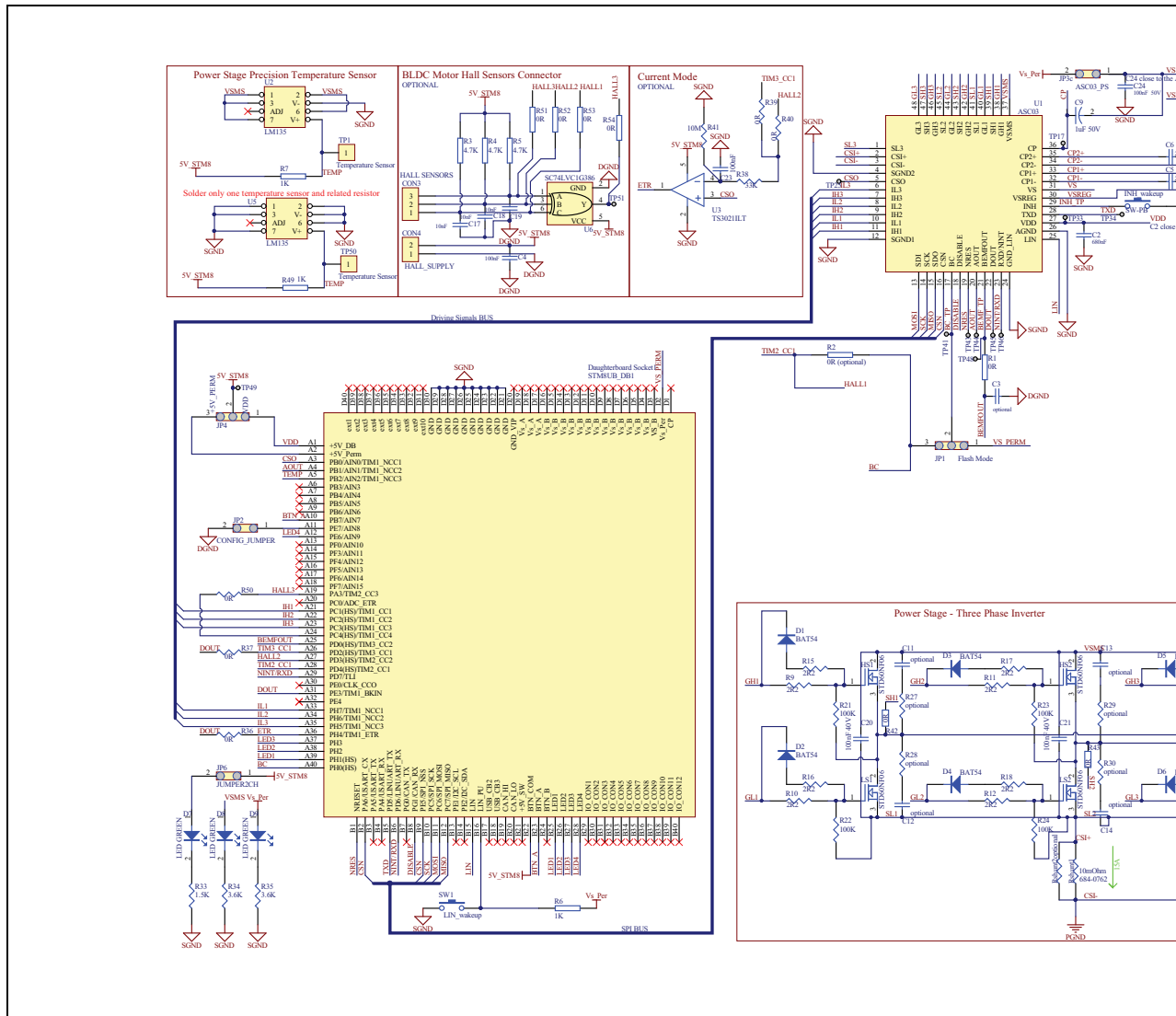
Figure 3. EVAL-L99ASC03 schematic
