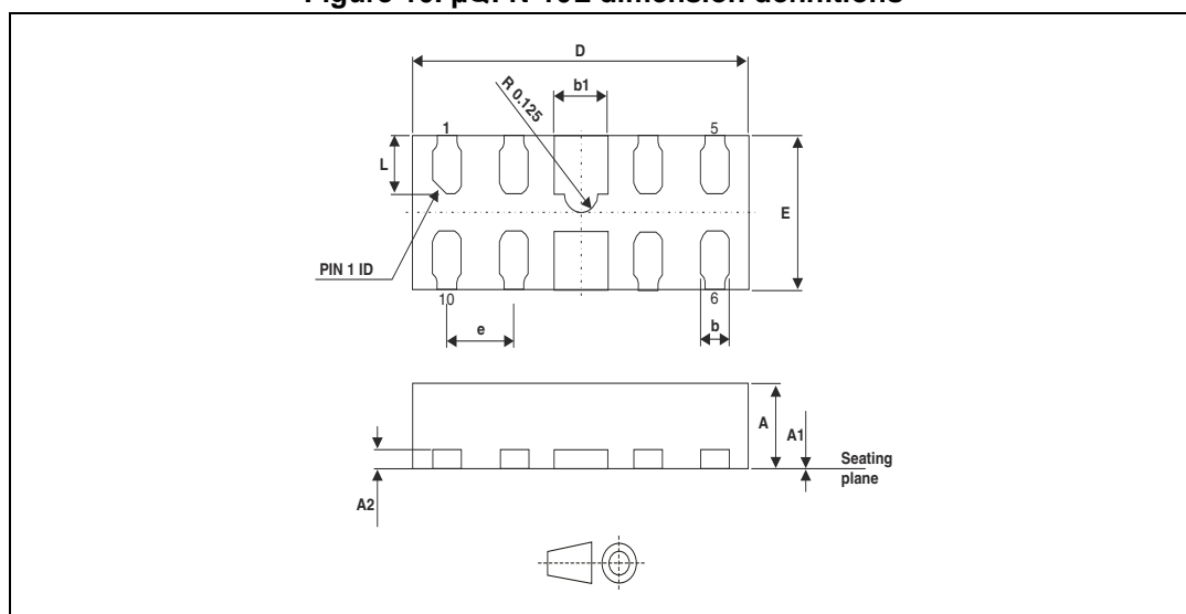
Figure 10. \mu QFN-10L dimension definitions
