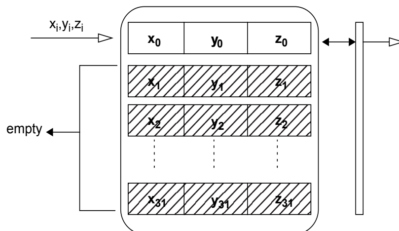
Figure 9. Bypass mode
