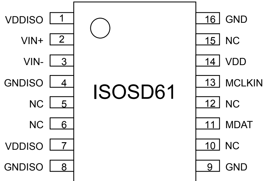
Figure 3. Pin connection
