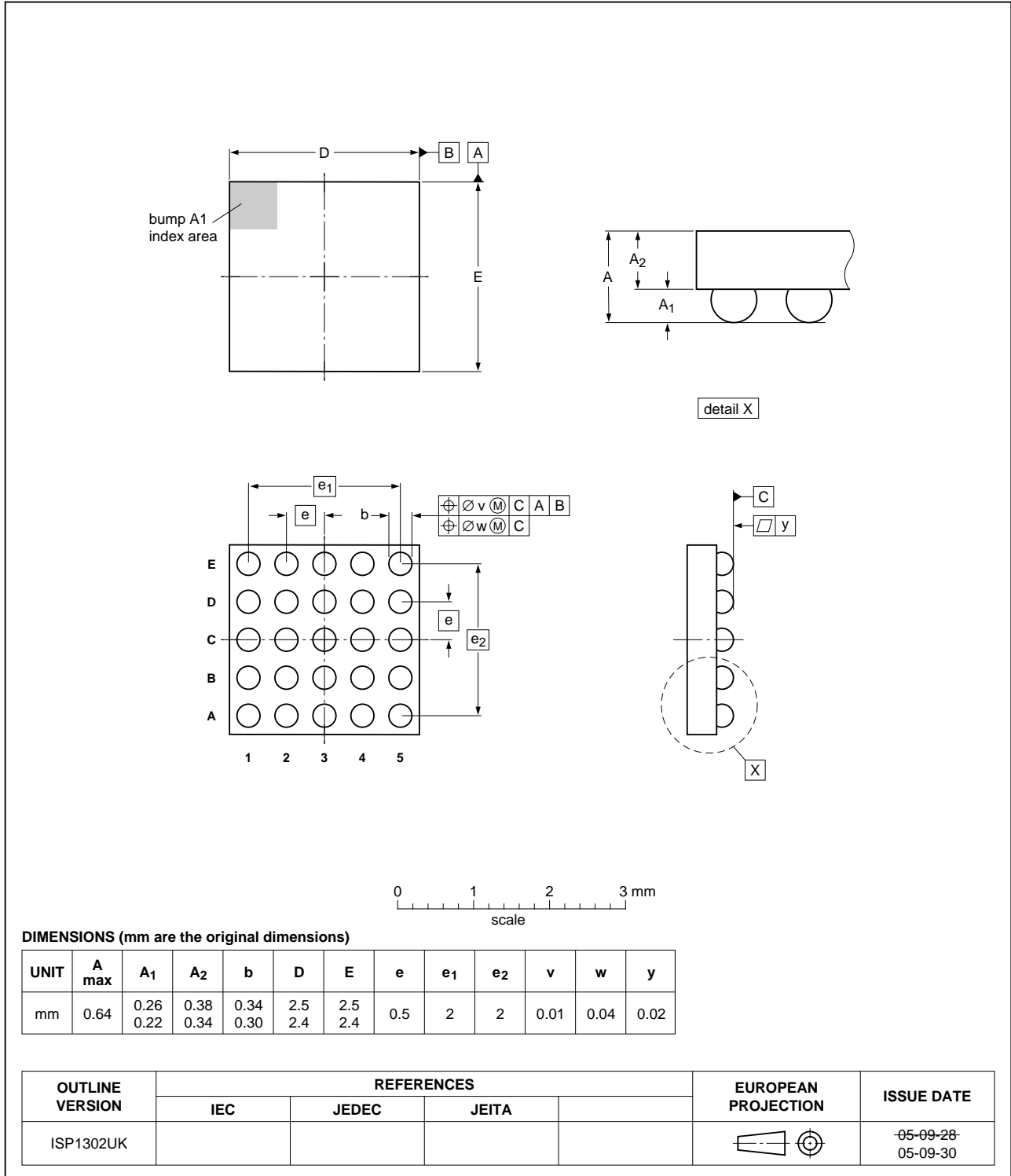
Fig 20. Package outline ISP1302UK (WLCSP25)
