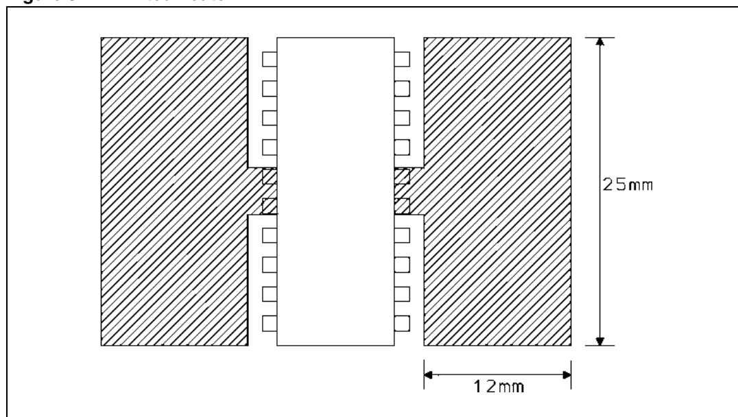
Figure 3. Printed heatsink
