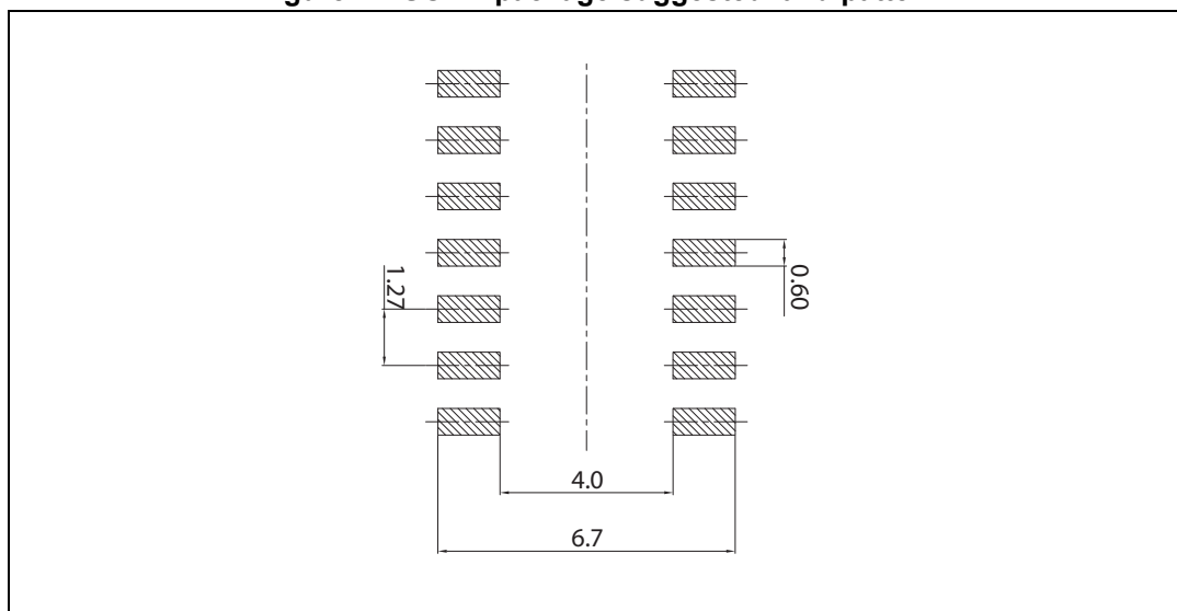
Figure 11. SO-14 package suggested land pattern
