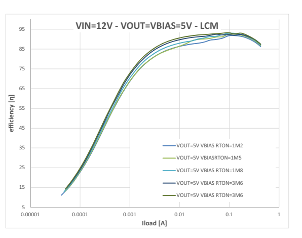
Figure 36. VIN 12 V - VOUT 5 V (log scale)
