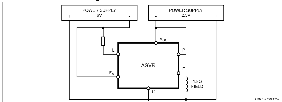
Figure 3. Reverse B+ test circuit
