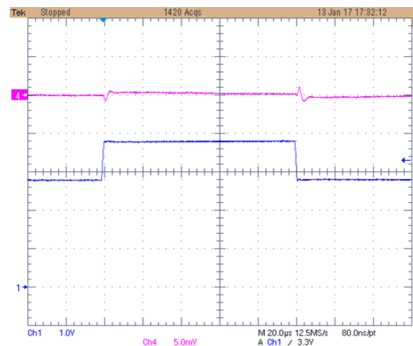
Figure 19. Line transient ( V_{OUT} = 1.8\text{ V}; I_{OUT} = 10\text{ mA}, t_r = t_f = 1\ \mu\text{s} )
