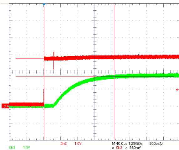
Figure 18. Turn-on Time ( V_{OUT} = 1.8\text{ V}; I_{OUT} = 0\text{ A}, V_{IN} = 2.8\text{ V}, t_r = t_f = 1\ \mu\text{s} )
