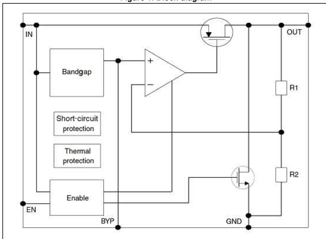
Figure 1. Block diagram
