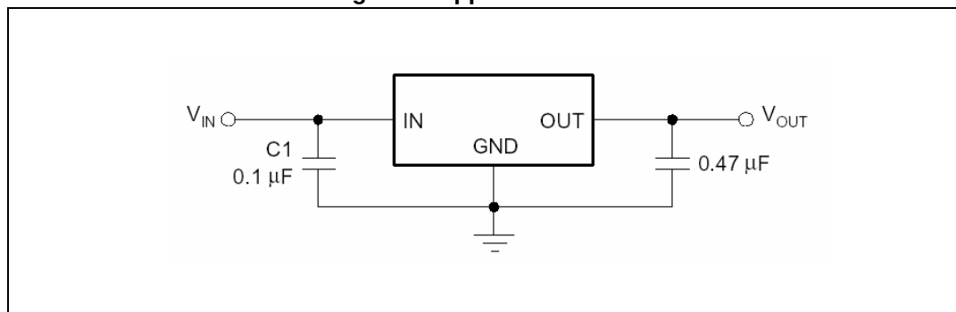
Figure 3. Application circuit
