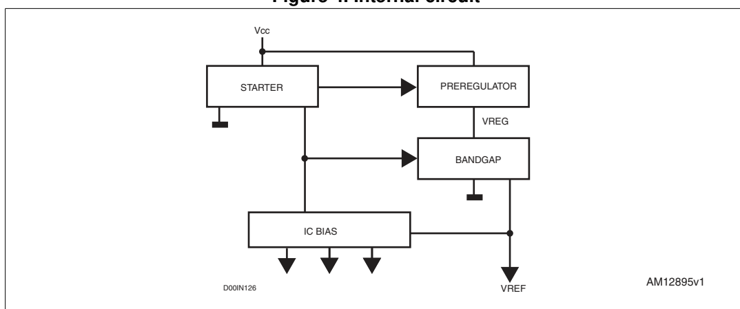
Figure 4. Internal circuit
