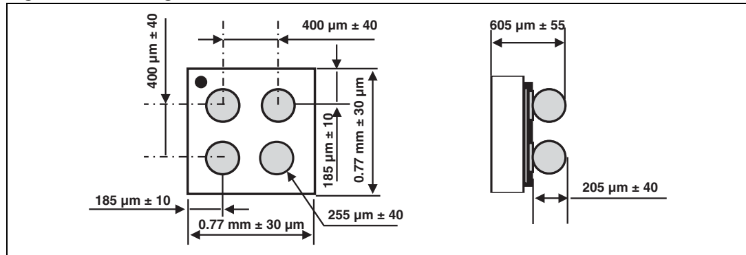
Figure 17. Package dimensions
