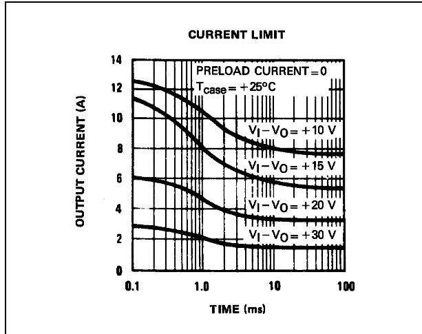
Figure 5. Current limit
