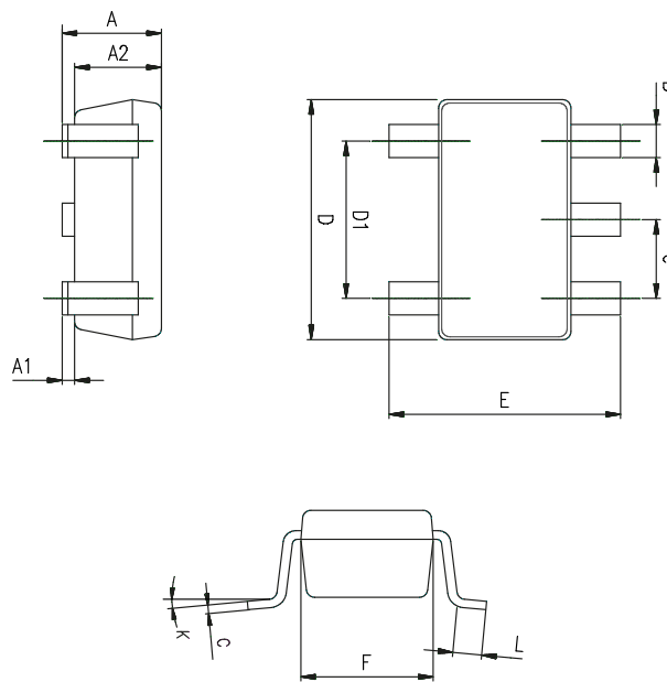
Figure 19. SOT23-5 package outline
