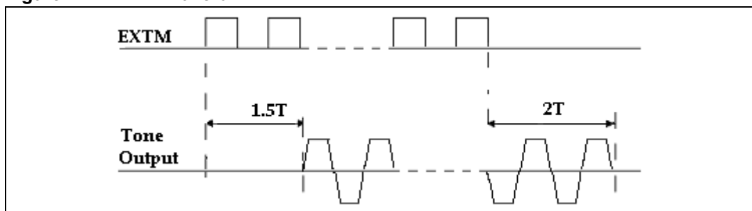
Figure 2. EXTM waveform
