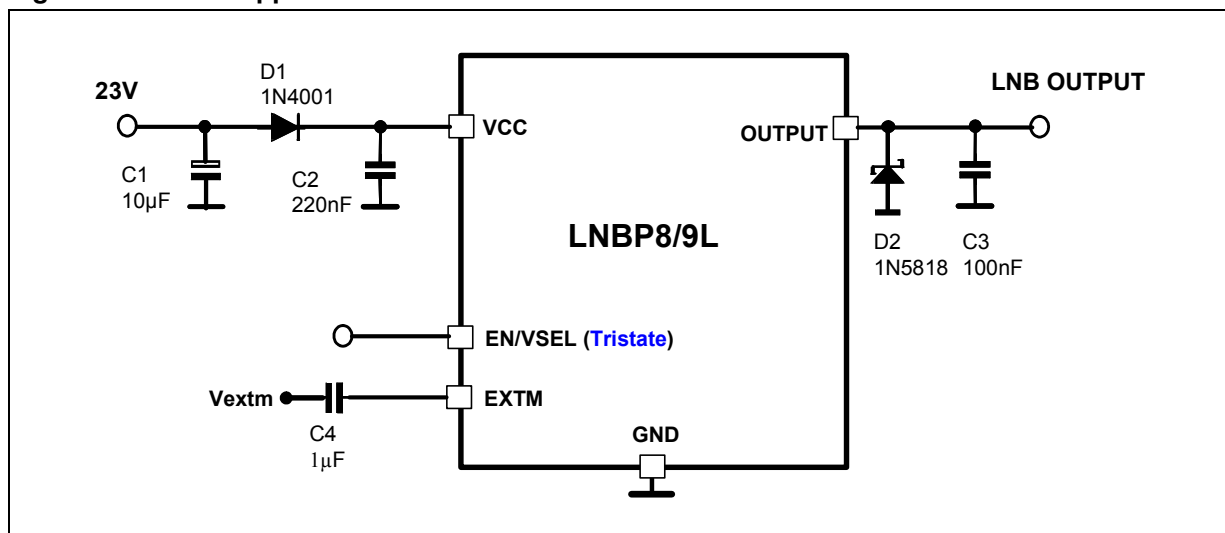
Figure 6. EXT TM application circuit
