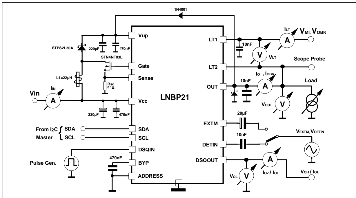
Figure 7: Test Circuit
