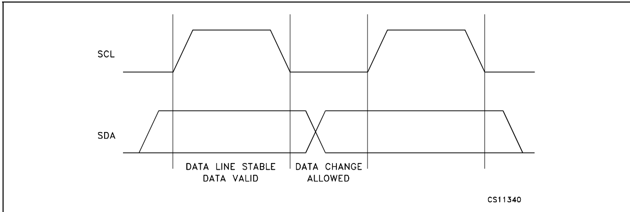
Figure 4: Data Validity On The I 2 C BUS
