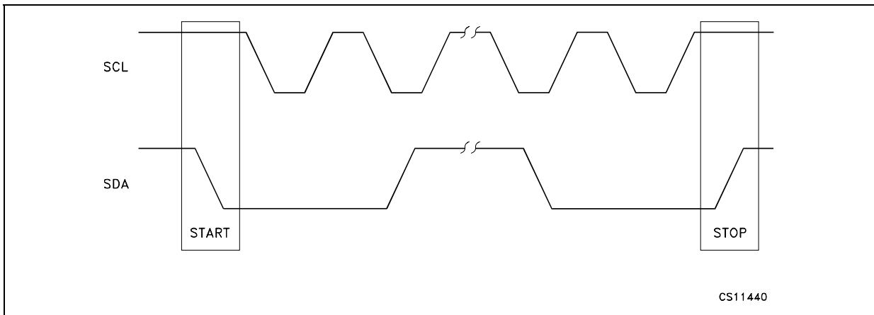
Figure 5: Timing Diagram On I 2 C Bus
