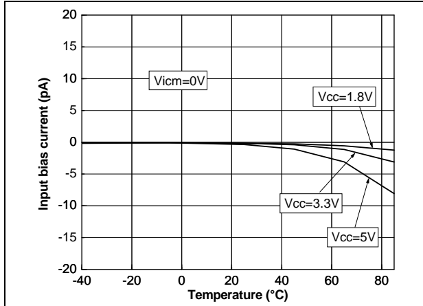
Figure 10. Input bias current vs. temperature at low V_{ICM}
