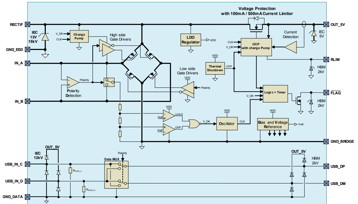
Figure 2. Functional diagram
