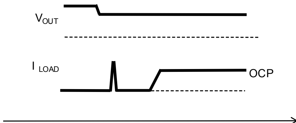
Figure 5. Fast overloading
