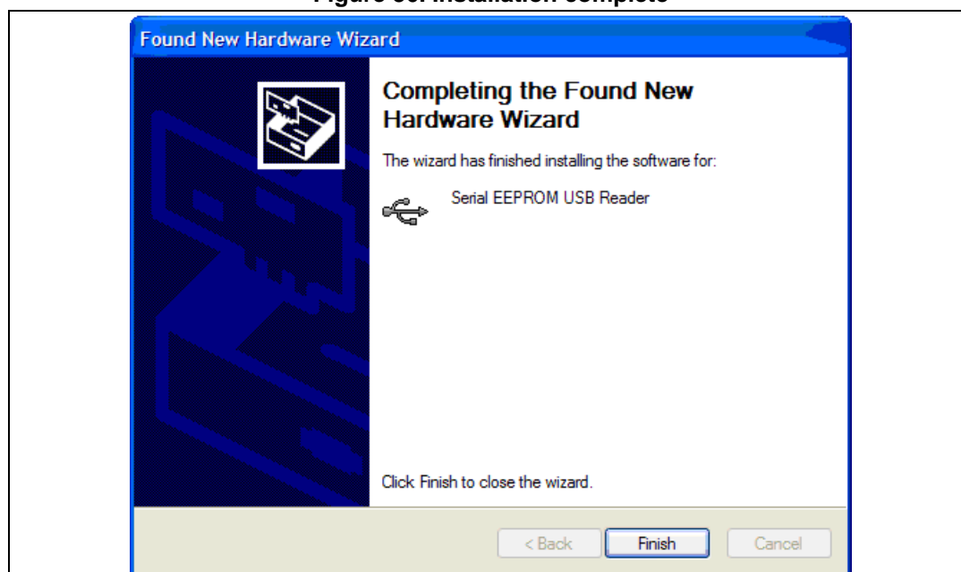
Figure 36. Installation complete
