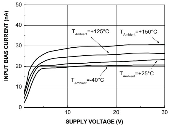
Figure 5. Input bias current
