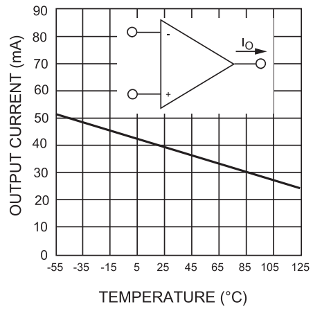
Figure 9. Current limiting
