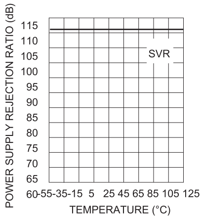
Figure 14. Power supply rejection ratio versus temperature
