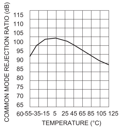
Figure 15. Common mode rejection ratio versus temperature
