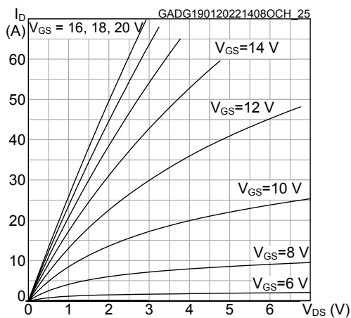
Figure 3. Typical output characteristics ( T_J = 25^\circ C )
