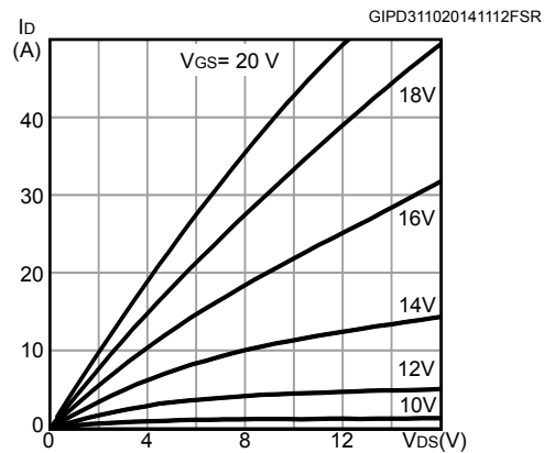
Figure 3. Output characteristics @ T_J = 25^\circ\text{C}
