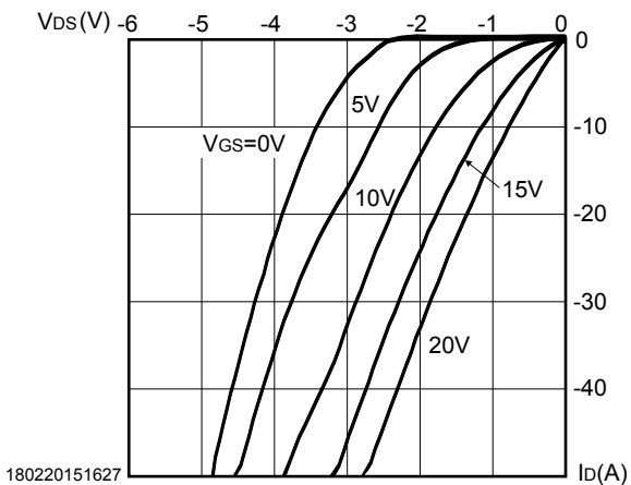
Figure 17. 3 rd quadrant characteristics ( T_J = 25^\circ\text{C} )
