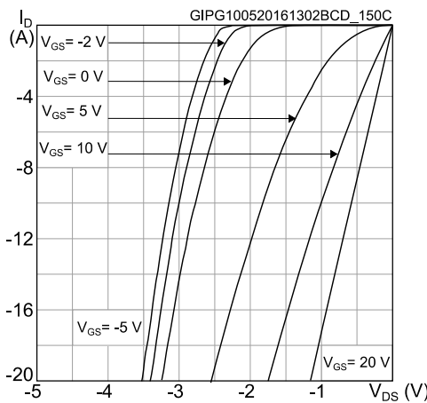
Figure 18: Reverse conduction characteristics ( T_J = 150 \text{ °C} )
