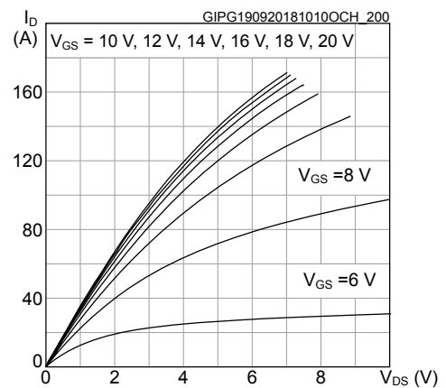
Figure 4. Output characteristics ( T_J = 200^\circ C )
