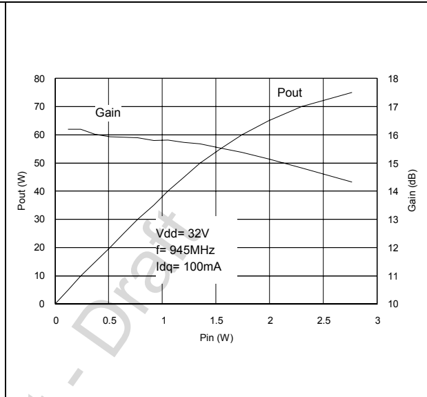
Figure 4. Output power and power gain vs input power
