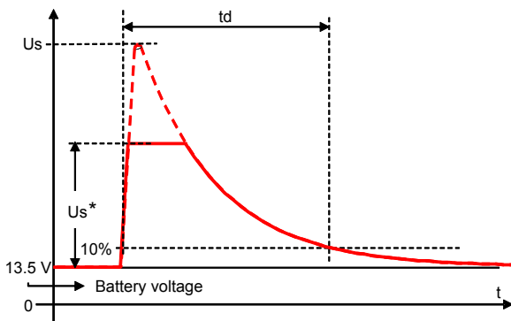
Figure 17. ISO7637-2 pulse 5b definition
