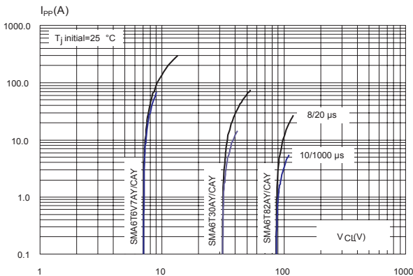
Figure 5. Maximum clamping voltage versus peak current exponential waveform
