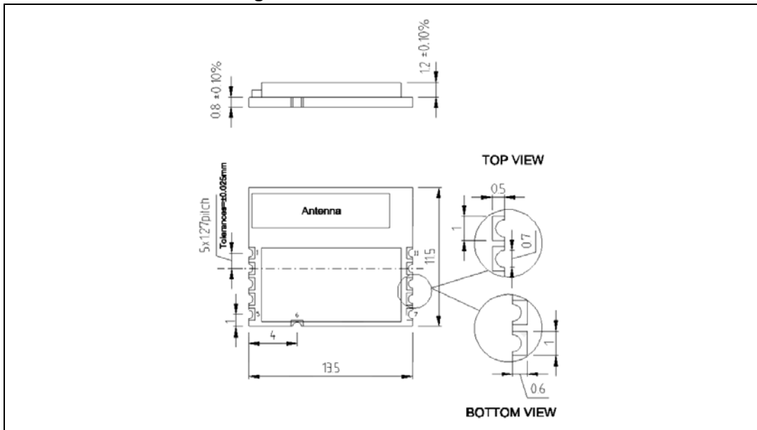
Figure 4. Mechanical dimensions
