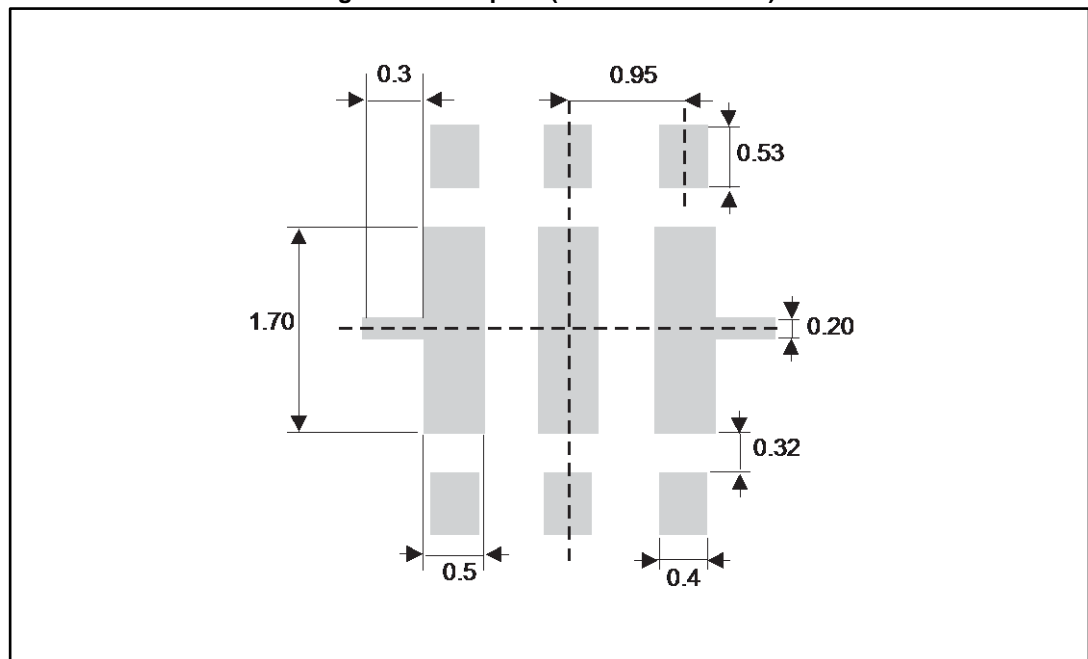
Figure 14: Footprint (dimensions in mm)
