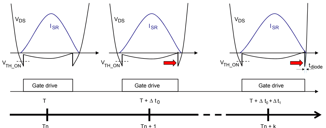
Figure 8. Adaptive turn-off
