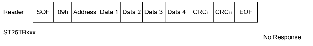
Figure 54. Write_block frame exchange between reader and ST25TB512-AC
