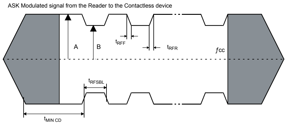
Figure 44. ST25TB512-AT synchronous timing, transmit and receive
