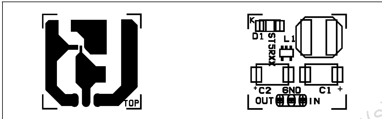
Figure 5: Typical Demoboard
