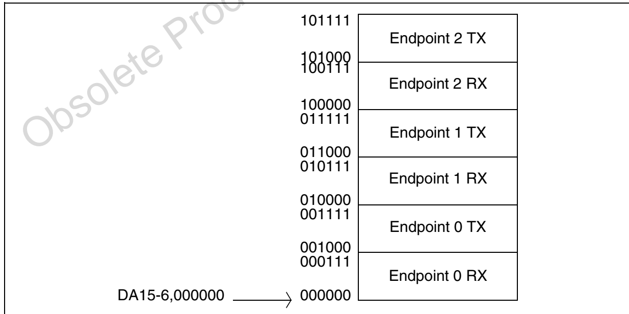
Figure 51. DMA Buffers
