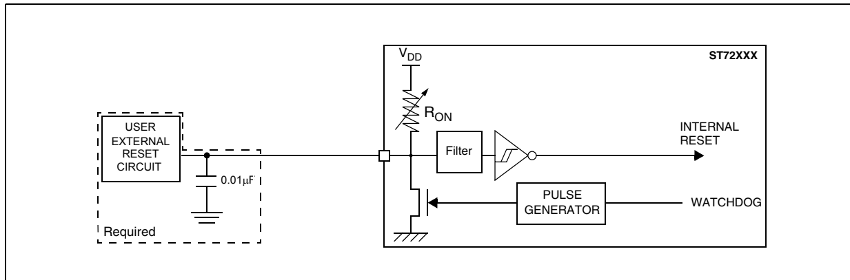
Figure 74. RESET pin protection when LVD is disabled
