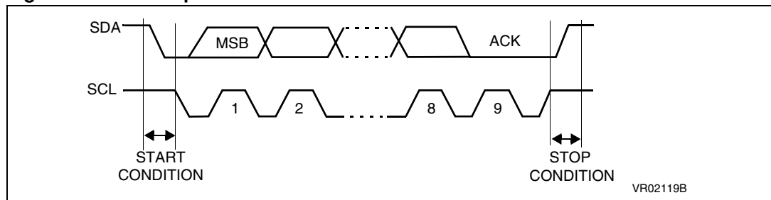
Figure 46. I 2 C bus protocol
