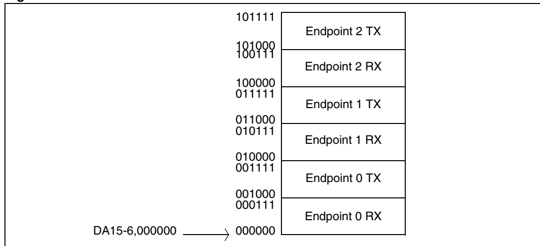
Figure 45. DMA buffers
