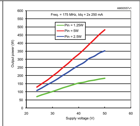
Figure 4. Output power vs drain supply voltage
