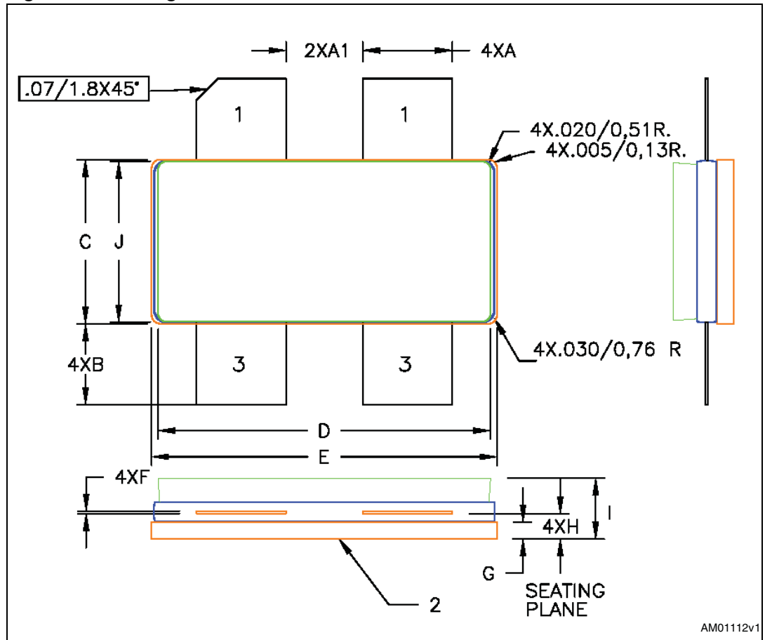
Figure 15. Package dimensions
