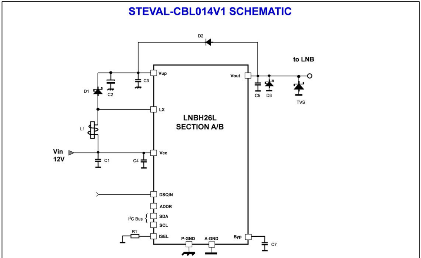
Figure 1: STEVAL-CBL014V1 schematic
