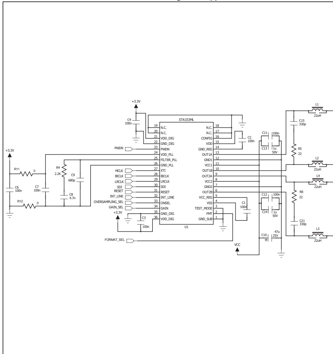
Figure 8. Application schematic
