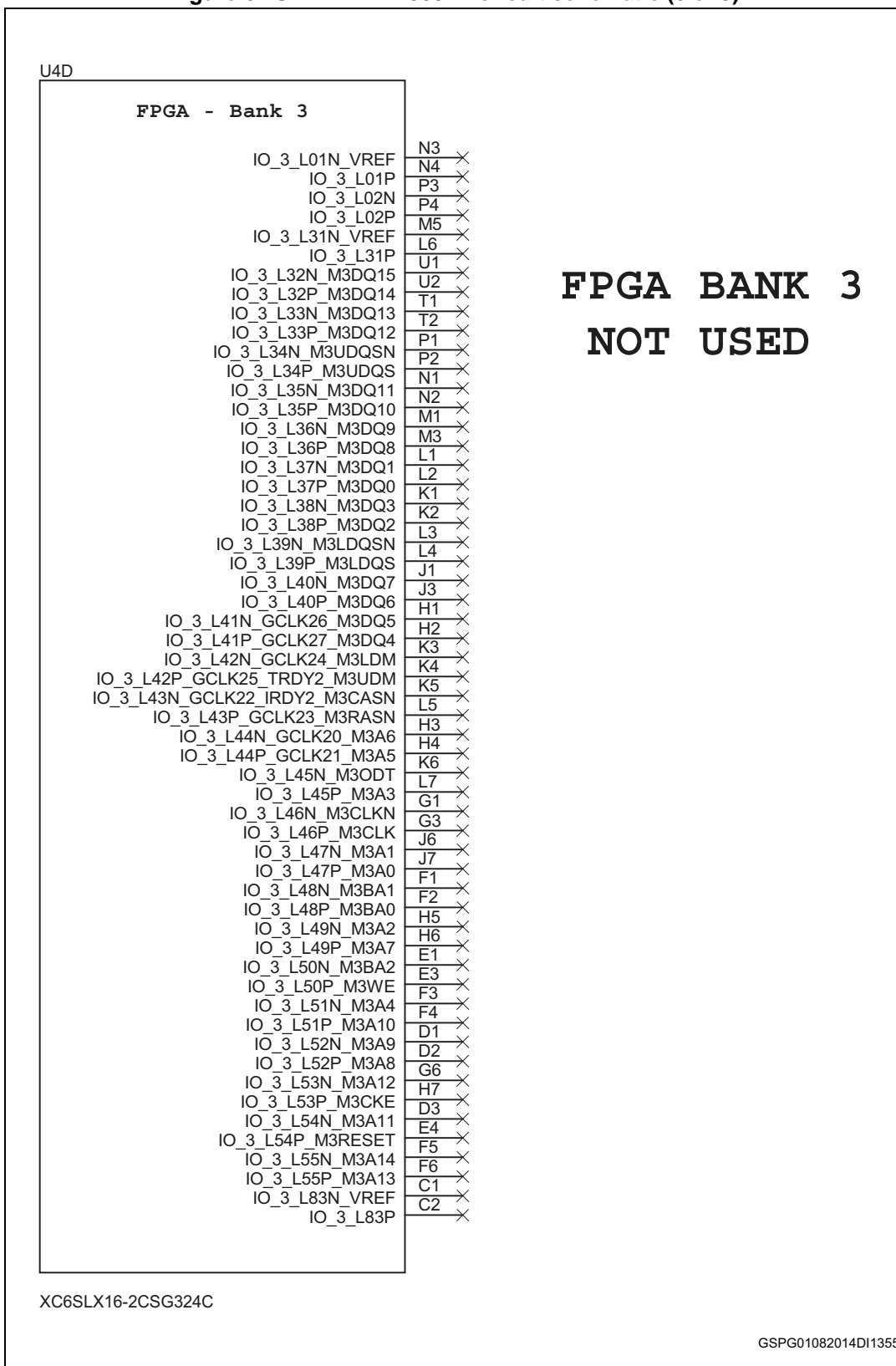
Figure 6. STEVAL-IME009V1 circuit schematic (6 of 9)
